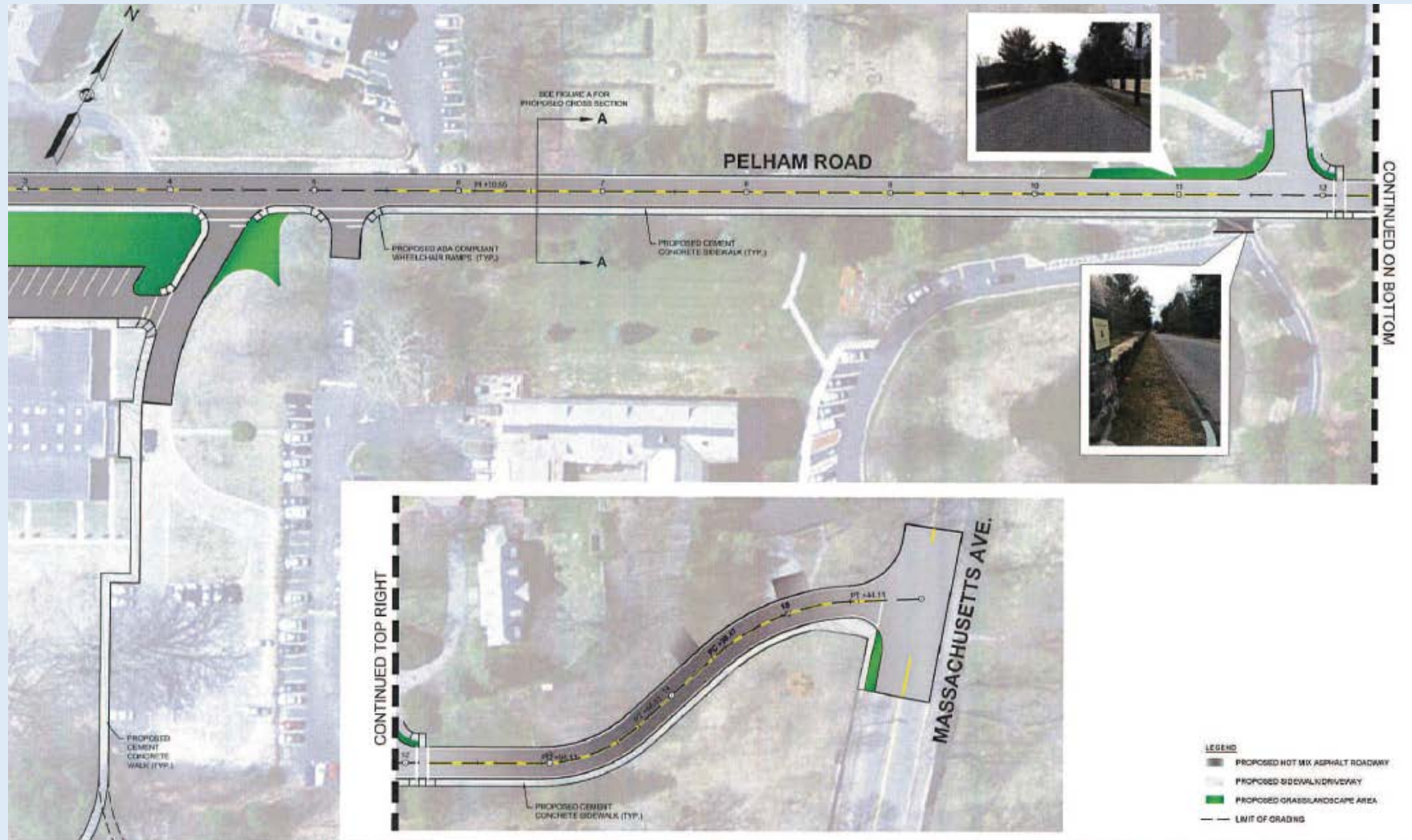
Sidewalk Installation along southerly side of Pelham Road
