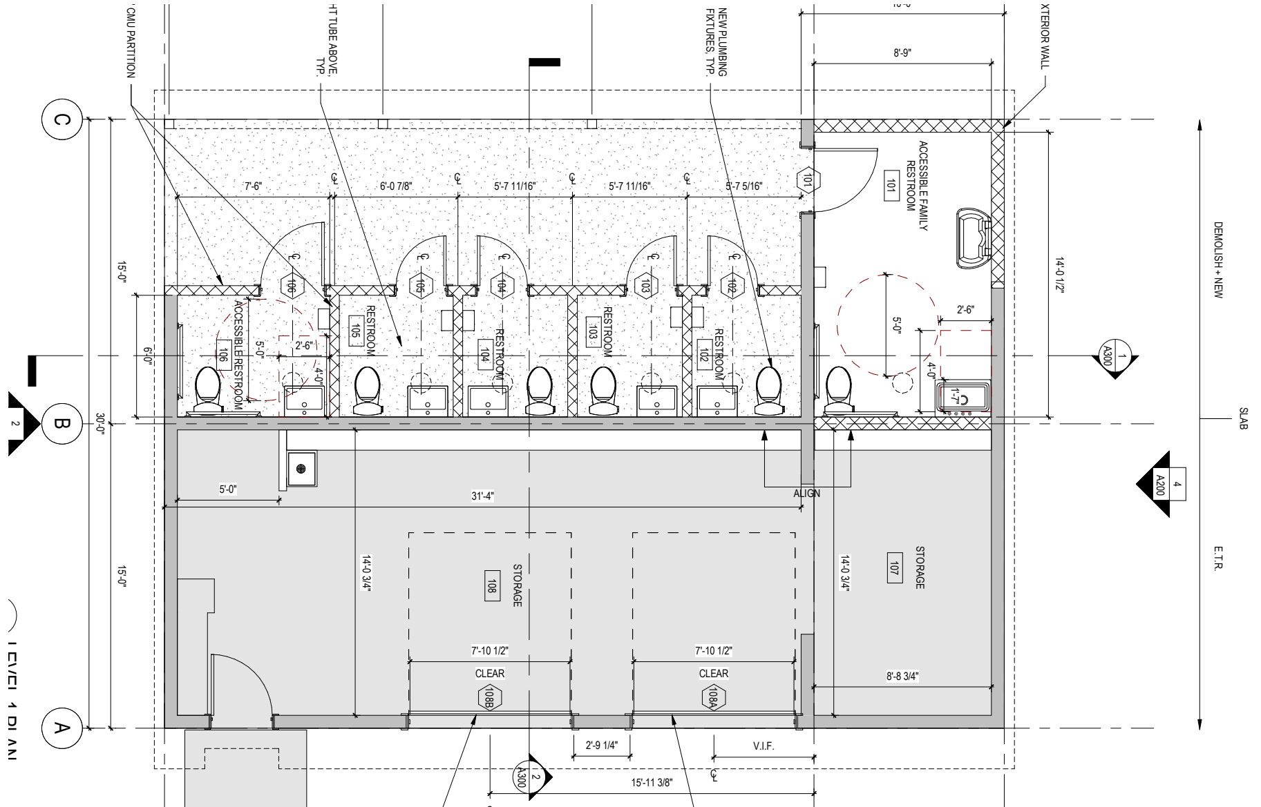
FLOOR PLAN
