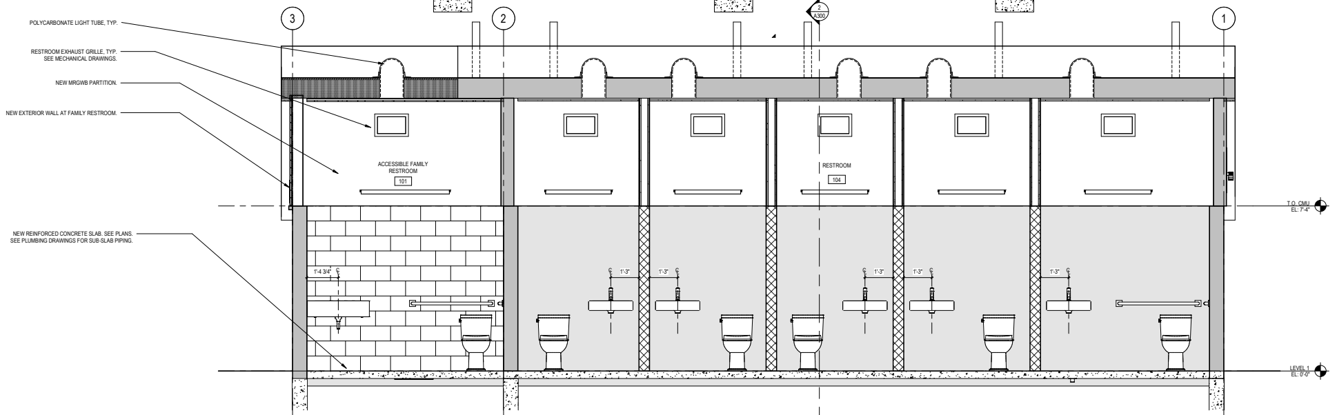
BUILDING CROSS SECTIONS
